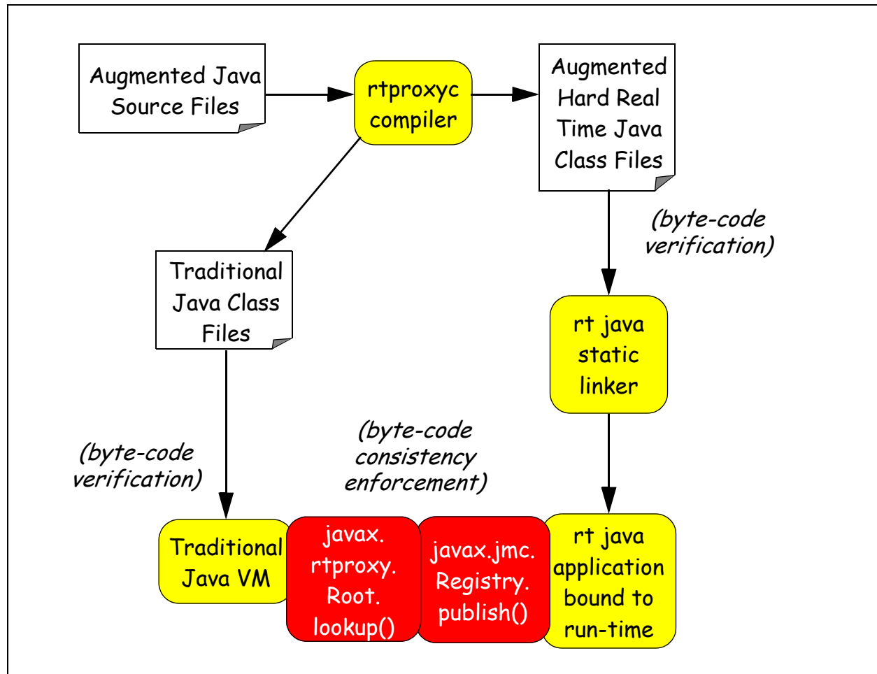
Figure 5: Compilation and Verification of Interface Components
